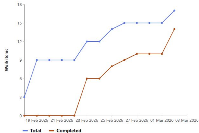
Burnup chart
