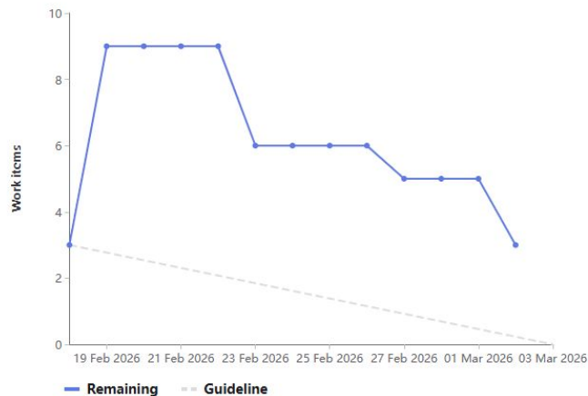
Burndown chart
